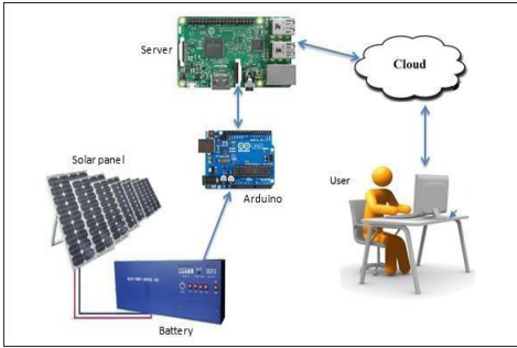
Fig 1. System Design
