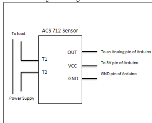
Fig 3. Current Sensor circuit
