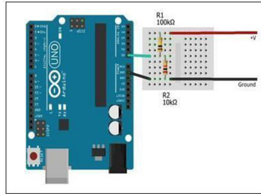
Fig 2. Voltage Divider
